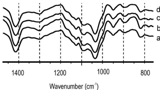
Figure 2. FTIR spectra (1470-750 \text{cm}^{-1} ) from alginate extracted from Eisenia arborea . Spectrum. a) alginate from stipes collected in November 2002, b) alginate from blades of November 2002, c) alginate from stipes of March 2003, d) alginate from blades of March 2003.
